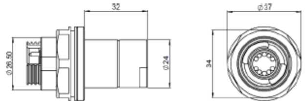
EUROLENS Receptacle Jam Nut Mount
