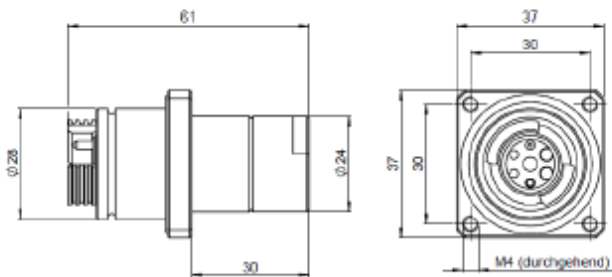
EUROLENS Receptacle Flange Mount
